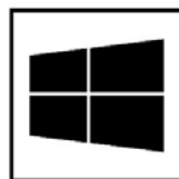
WINDOWS 8
