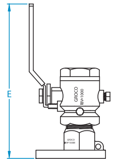
IBV MOUNTED ON IBVF
