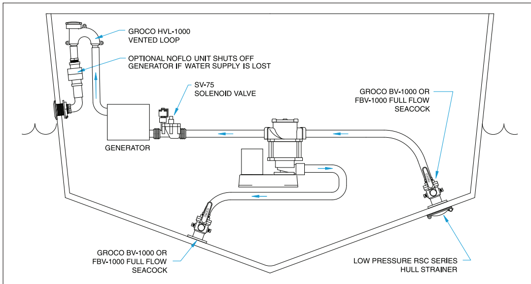
911 SAMPLE INSTALLATION
