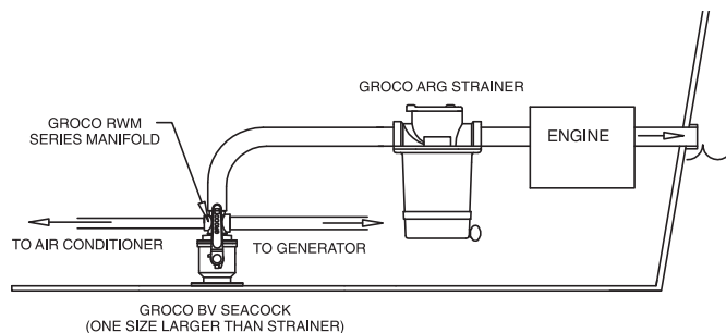
Sample Installation shows RWM Manifold used to distribute raw (unfiltered) water
