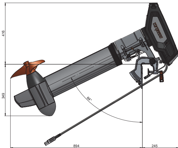
Tilt Position 4 Tilt position 4 Cruise 3/6 RL
