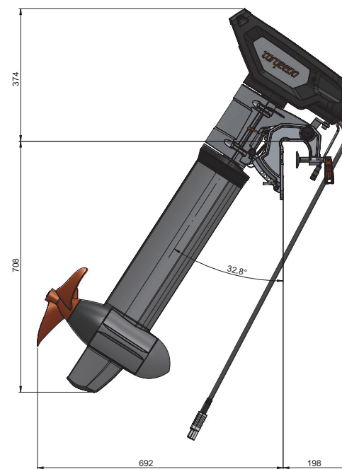
Tilt Position 2 Tilt position 2 Cruise 3/6 RL
