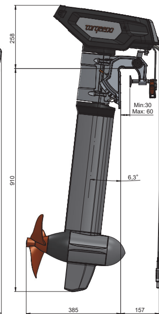
Tilt Position 1 Tilt position 1 Cruise 3/6 RL
