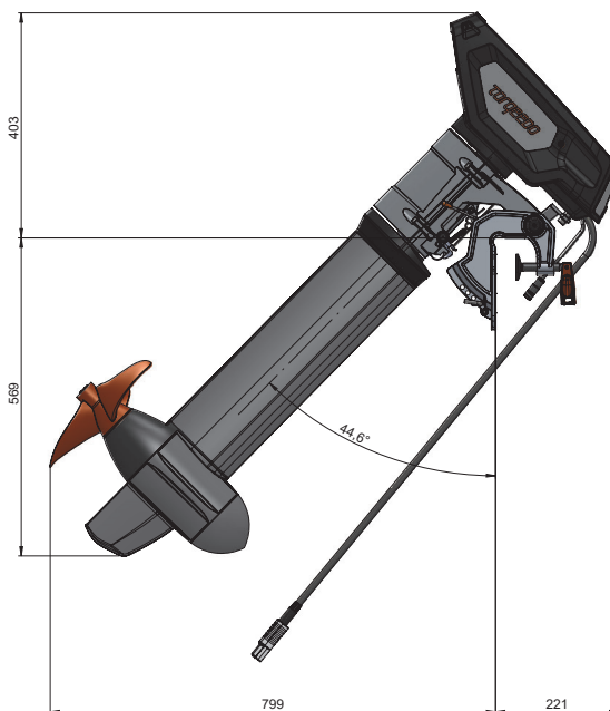
Tilt Position 3 Tilt position 3 Cruise 3/6 RL
