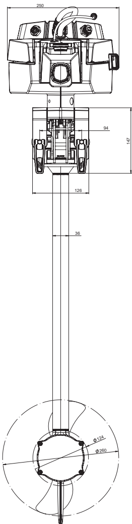
Front View / Frontalansicht
