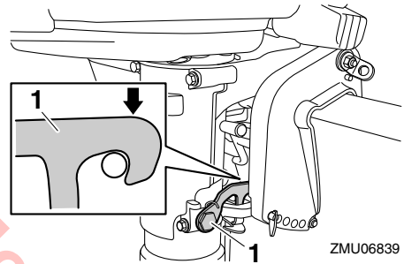
1. Tilt lock
