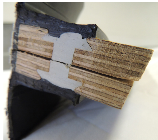
Single rivet cross section
