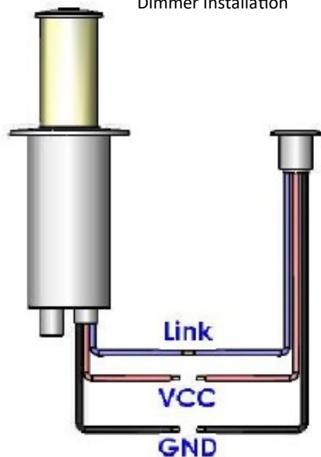
Dimmer Installation
