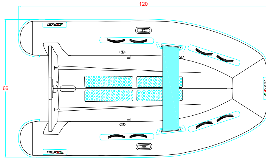
PLANT VIEW VISTA SUPERIOR
